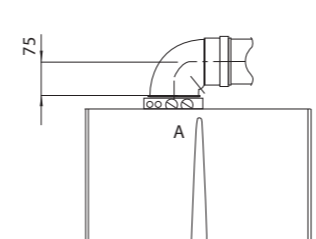
Kit coaxial orizontal Ø60/100
